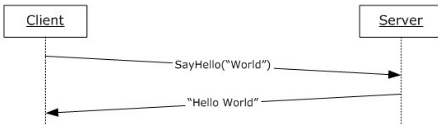
Figure 1: Middleware Protocol
