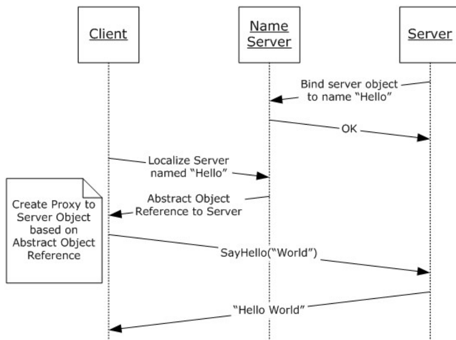
Figure 3: Binding a server object to the logical name "Hello" in the name server
