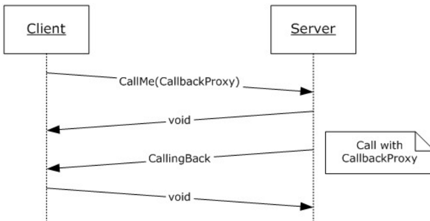
Figure 2: An abstract object reference sent by the protocol client and then used by the protocol server to call back the protocol client
