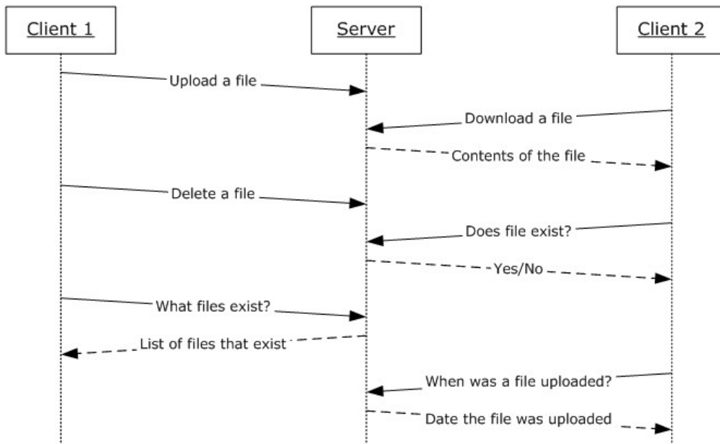
Figure 1: Communication between protocol clients and protocol server
