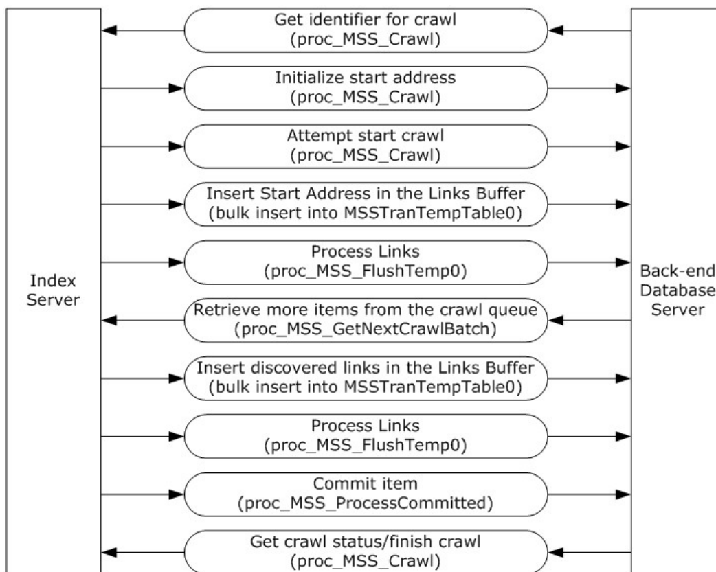
Figure 1: Flow of data during a full crawl operation
