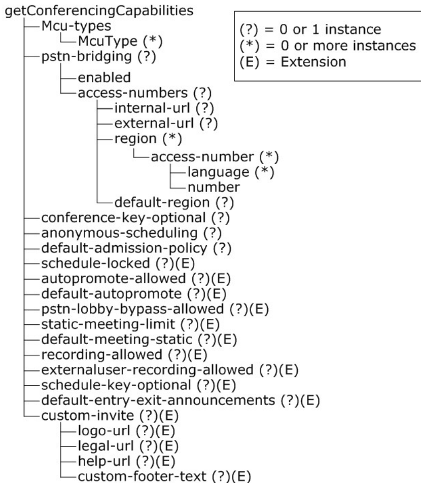
Figure 15: getConferencingCapabilities element hierarchy
