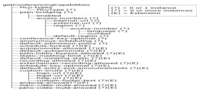
Figure 12: getConferencingCapabilities element hierarchy
