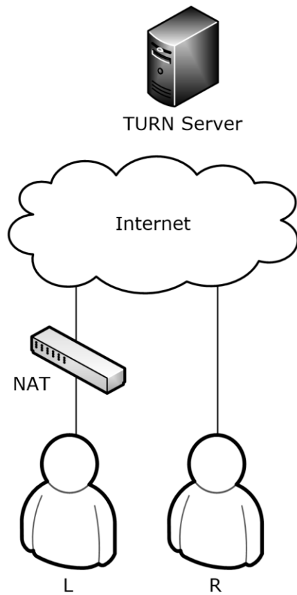
Figure 3: ICE implementations
